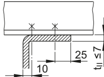
Cold-formed shapes
