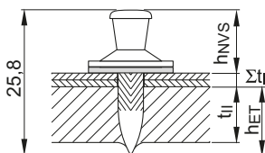
Nail for X-HVB composite connector X-ENP-21 HVB
